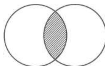
図1. AND 検索
